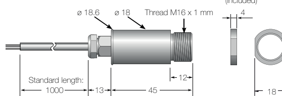
Sensing Head
