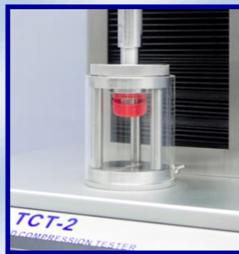
TCT-2 for Tamper Evident band breaking test (with optional fixture)
